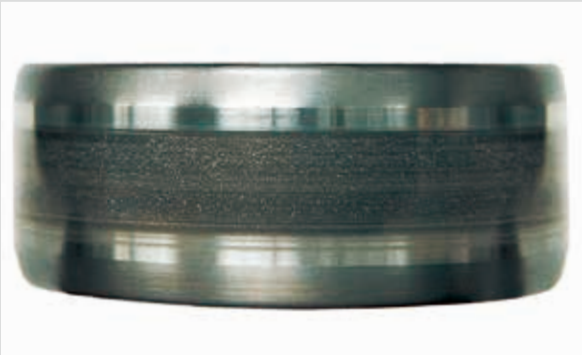
Photo 9 Part: Inner ring of a cylindrical roller bearing Symptom: Belt pattern of electrical erosion accompanied by pits on the raceway surface
